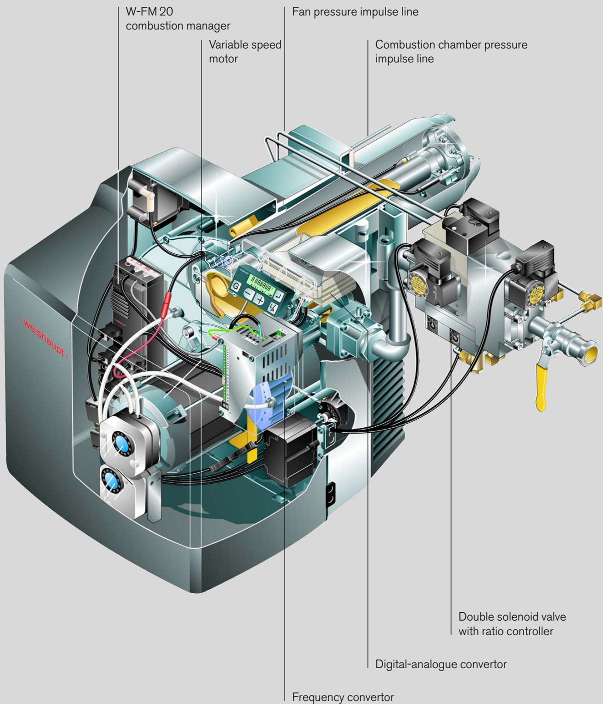
Example: WG40 with speed control
