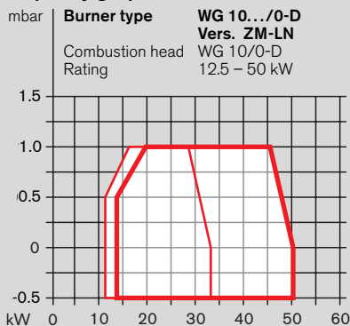
Capacity graph WG 10
