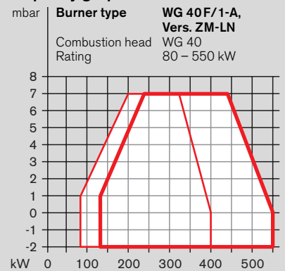
Capacity graph WG 40
