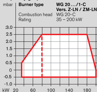
Capacity graph WG 20
