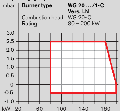
Capacity graph WG 20
