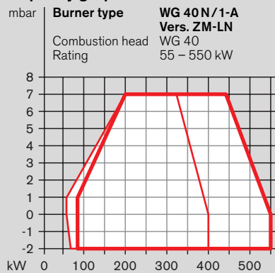
Capacity graph WG 40
