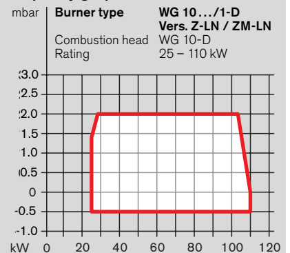
Capacity graph WG 10
