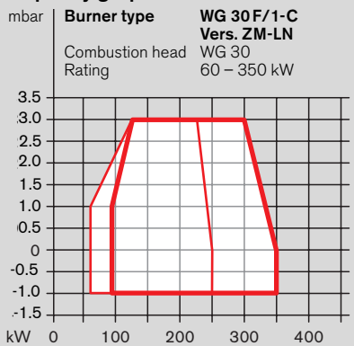
Capacity graph WG 30
